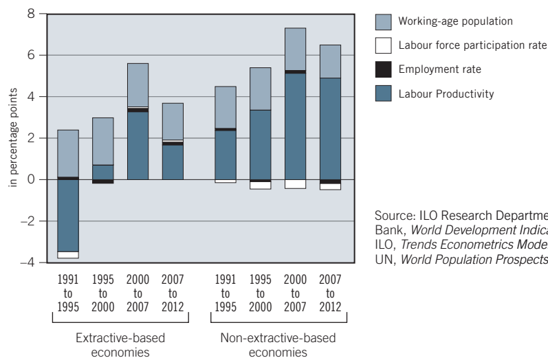
Figure 3.7 Productivity decomposition
